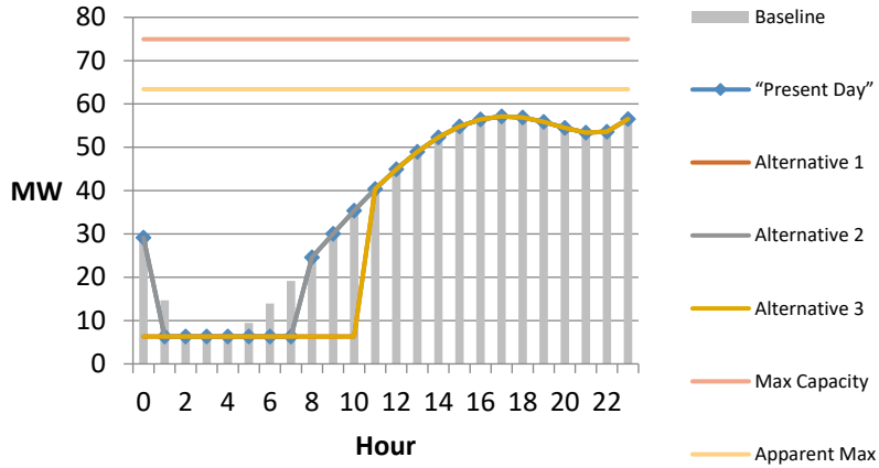
Carribou1 - August Weekend Power Profile
