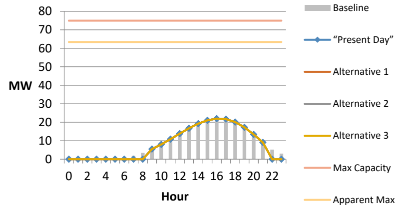
Carribou1 - Late September Weekend Power Profile
