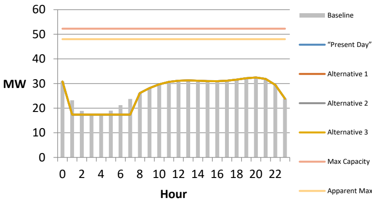
Butt Valley - Late September Weekend Power Profile
