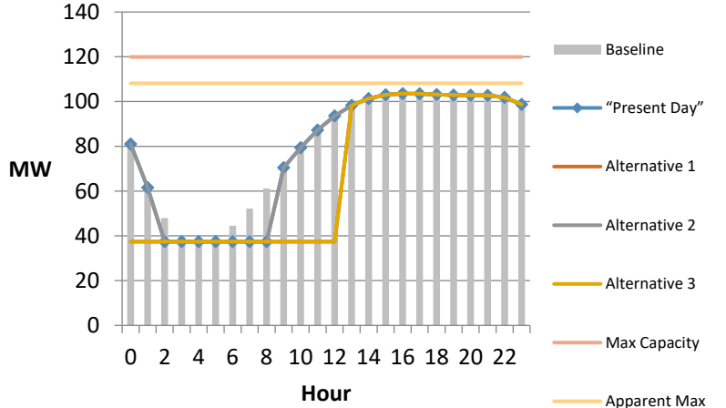
Carribou2 - August Weekday Power Profile
