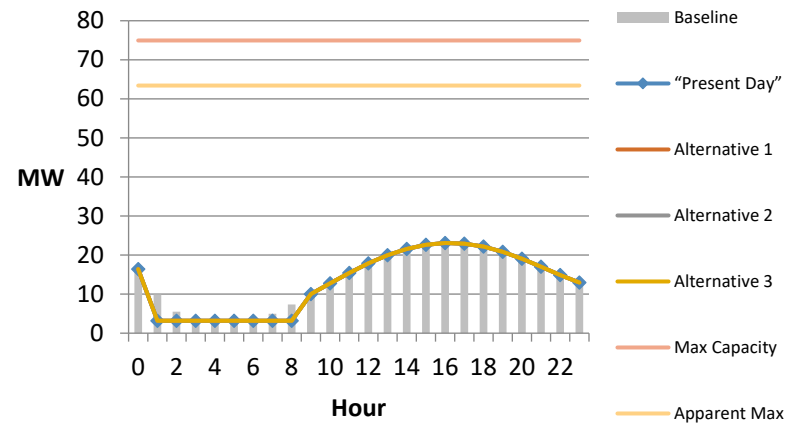
Carribou1 - Late September Weekday Power Profile
