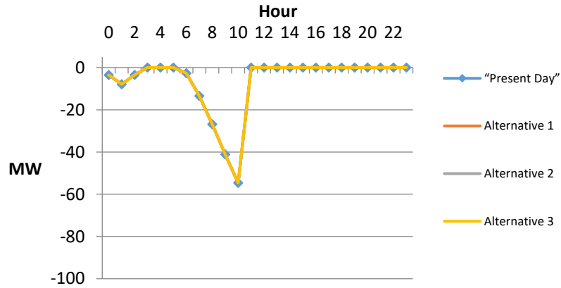
Carribou2 - Early June Weekend Power Changes
