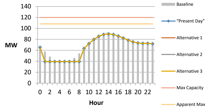
Carribou2 - Late September Weekday Power Profile
