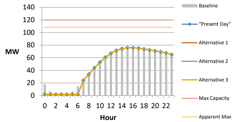
Carribou2 - Early June Weekday Power Profile
