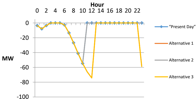
Carribou2 - Late June Weekend Power Changes
