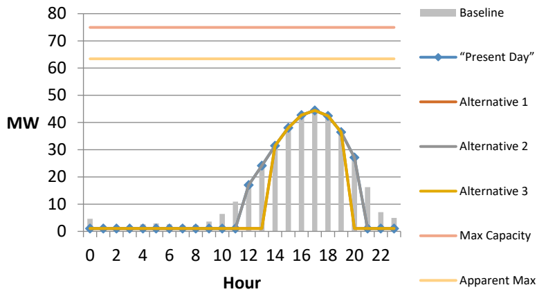
Carribou1 - Late June Weekday Power Profile
