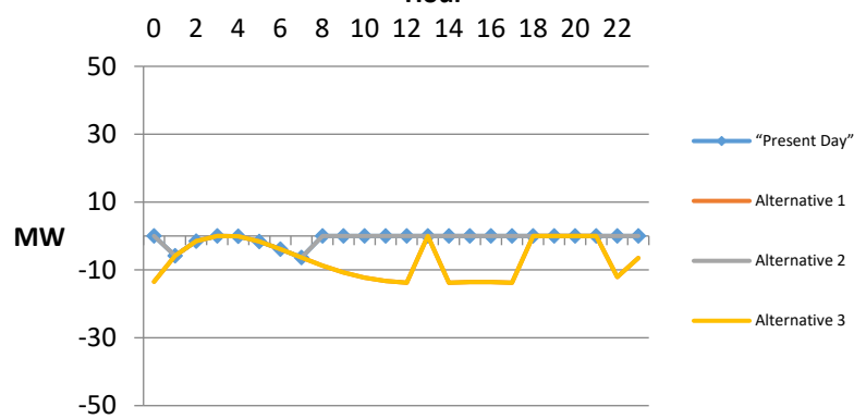
Butt Valley - Early September Weekend Power Changes
