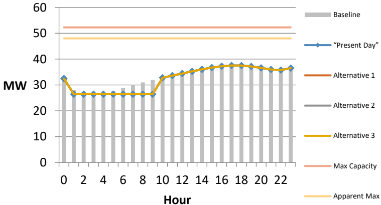
Butt Valley - Late September Weekday Power Profile
