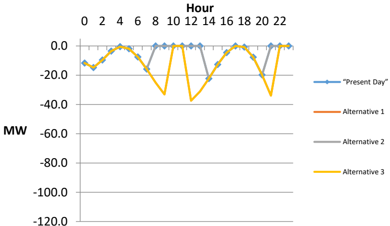
Carribou2 - Late June Weekend Power Changes
