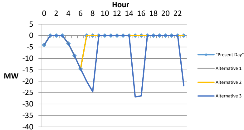
Butt Valley - August Weekday Power Changes
