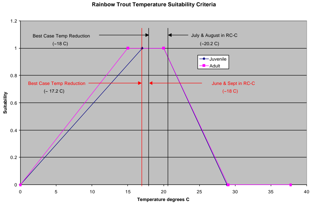
Figure 1. Adult and juvenile rainbow trout Temperature Suitability Curve for first five-year flow release schedule for Rock Creek –Cresta reaches (temperature lines fitted by eye).
