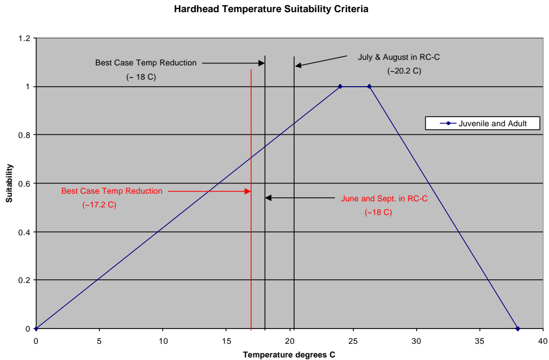
Figure 2. Hardhead Temperature Suitability Curve for first five-year flow release schedule for Rock Creek-Cresta reaches (temperature lines fitted by eye).
