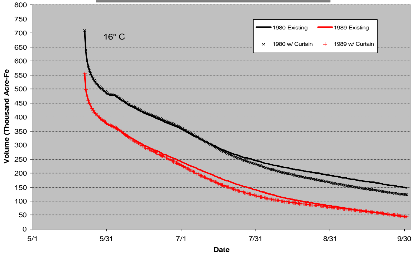
Comparison of Top and Bottom Envelopes of 16 C Cold-Water Depletion Rates With and Without Prattville Intake Modification Envelope of All Normal Years in 1970-2002
