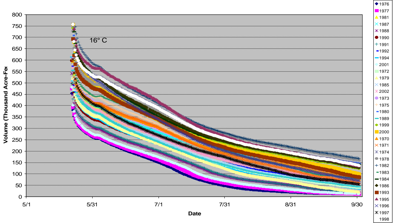
Available Volume of Water with Temperatures Lower than the Specified Level in Lake Almanor, Existing Conditions, 1970-2002
