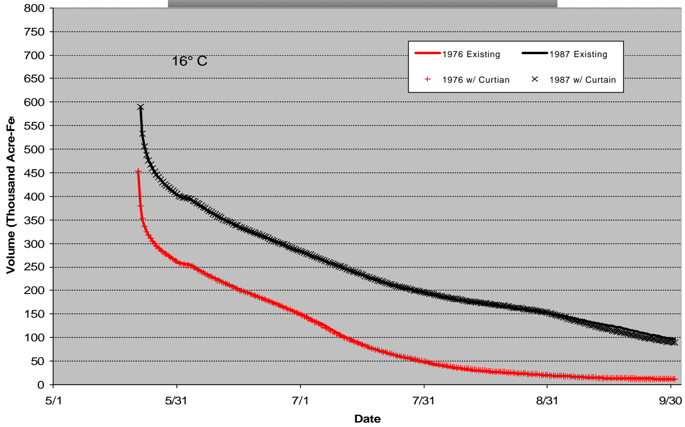
Comparison of Top and Bottom Envelopes of 16 C Cold-Water Depletion Rates With and Without Prattville Intake Modification Envelope of All Critical Dry Years in 1970-2002
